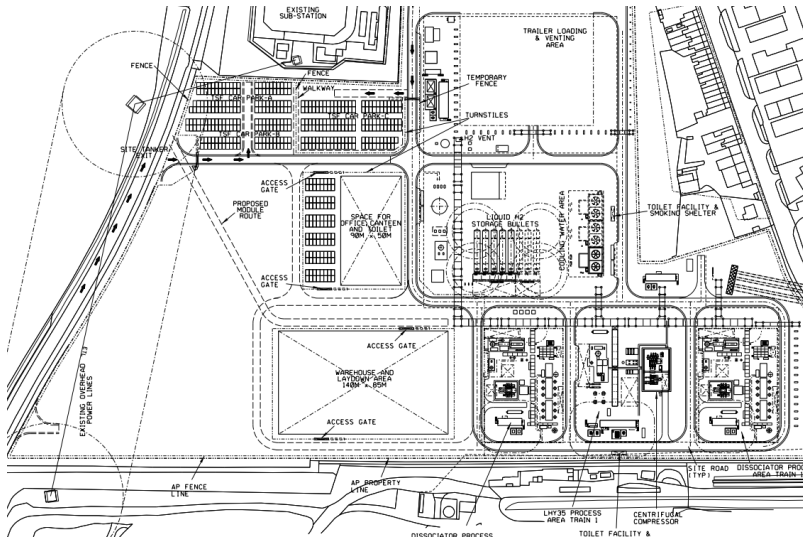
Plate 1-2: Illustrative layout of Work No. 7 during temporary use
