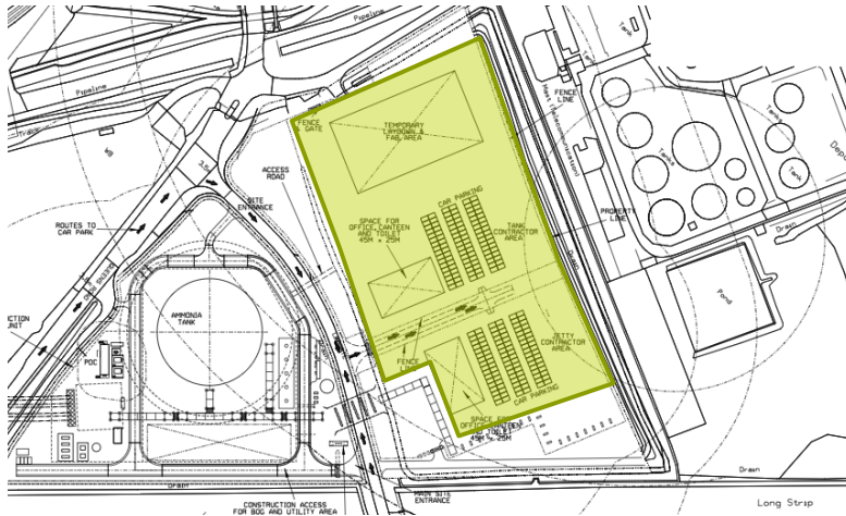
Plate 1-1: Illustrative layout of area of Work No. 5 during temporary use
