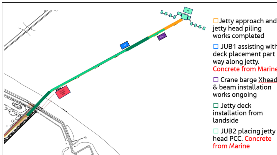
Plate 1-5: Example landside and marine construction sequence
